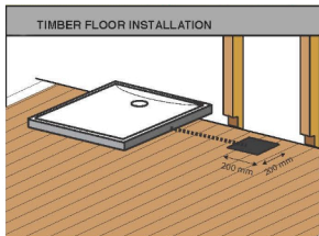
A. TIMBER FLOOR
