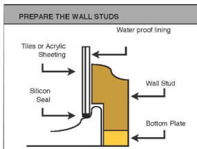
RECOMMENDED METHOD FOR FITTING SHOWER BASE
